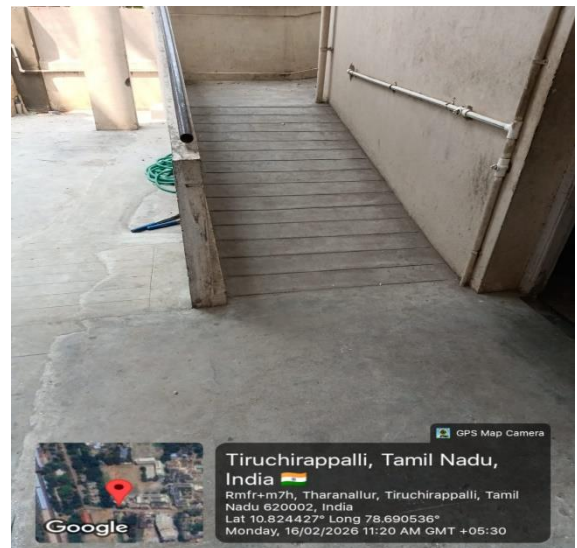
Ramp in Blossoms Special School
